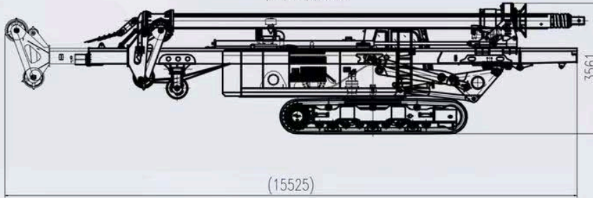
YCR160D旋挖钻机性能参数(516F01)
